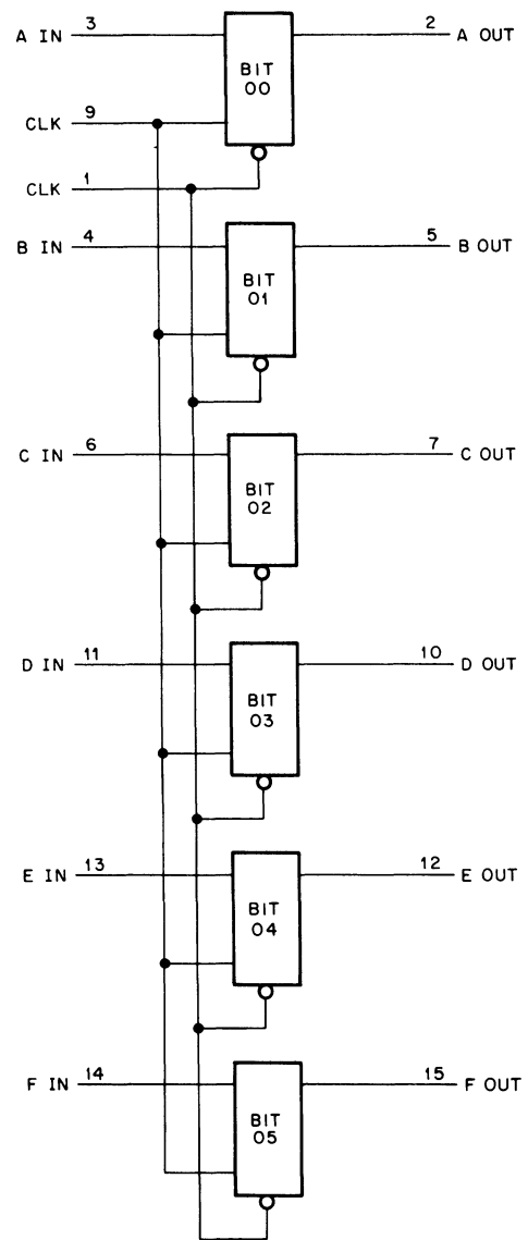
Figure 5-4 IC 74174 – Simplified Logic Diagram
