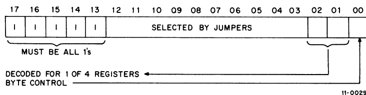
Figure 5-2 Controller Select Address Format
