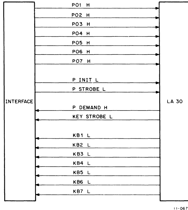
Figure 5-5 Interface Signals
