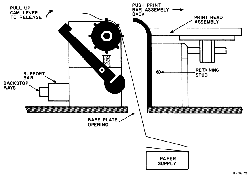
Figure 3-2 Loading Paper into LA30 DECwriter
