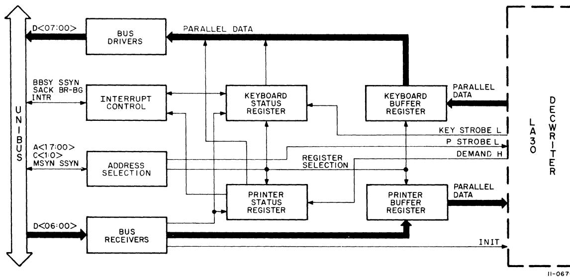
Figure 2-1 LC11 Controller – Simplified Block Diagram
