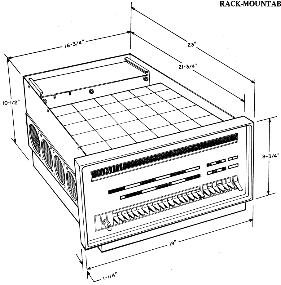
Overall Dimensions
