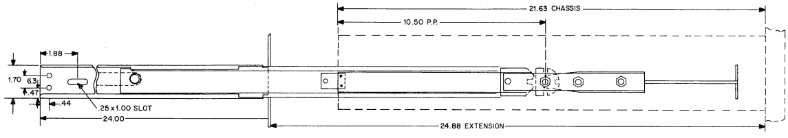
Side View of Mounting Hardware
