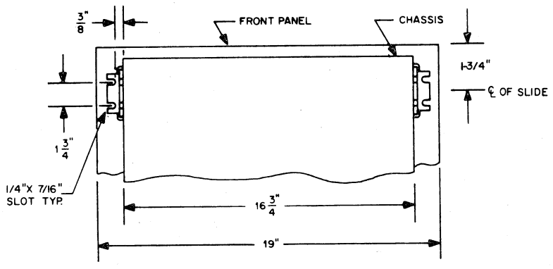
Rear View of Mounting Hardware
