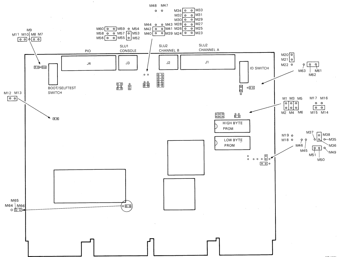
Figure 2-1 KXJ11-CA Jumper Layout
