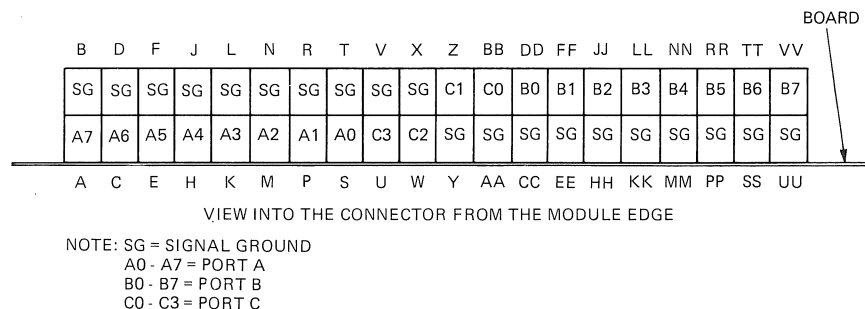
Figure 5-1 Parallel I/O Interface Pin Assignments
