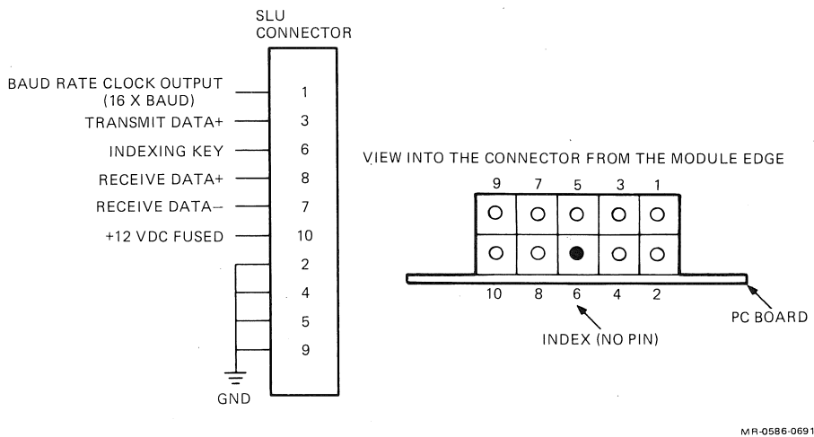
Figure 5-2 J2 and J3 Pin Assignments (10-Pin)
