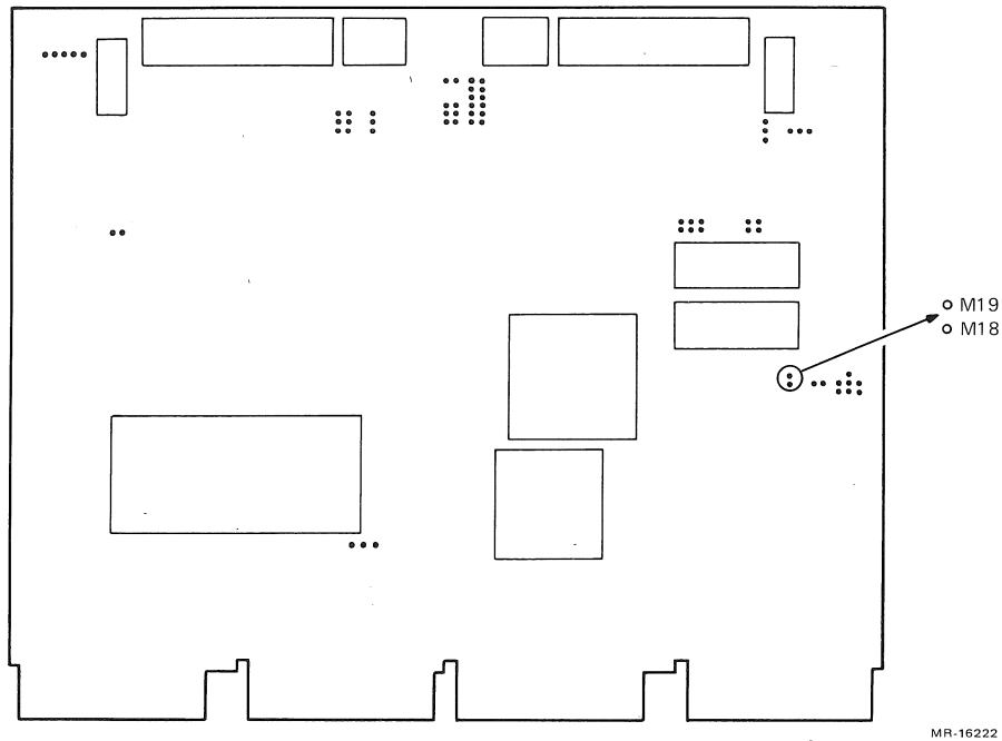
Figure 2-12 PROM Addressing
