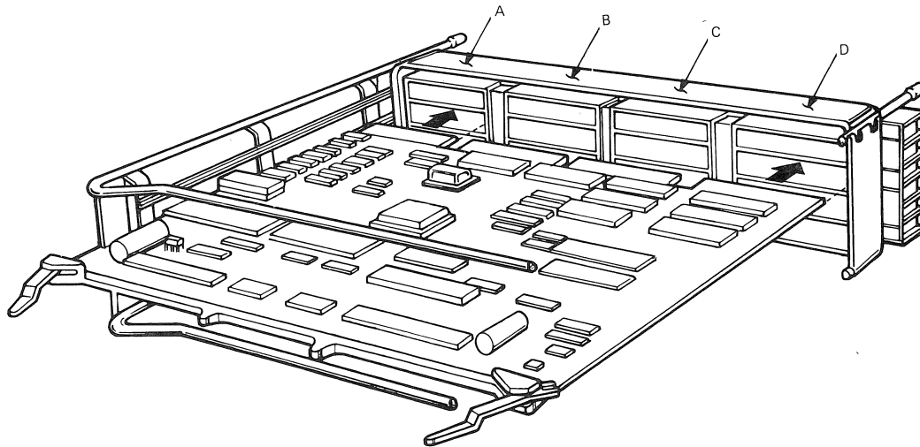
Figure 4-1 Backplane Installation
