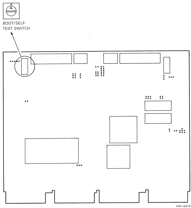
Figure 2-4 Boot/Self-Test Switch
