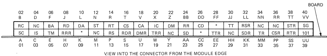
Figure 5-3 J1 Pin Assignments (40-Pin)
