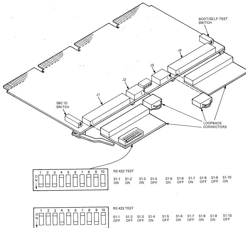
Figure 5-4 Loopback Connectors
