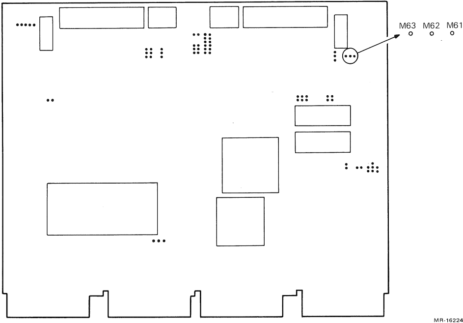
Figure 2-14 SLU1 Transmitter
