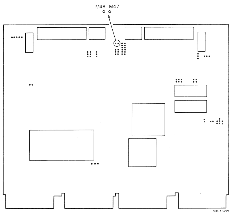
Figure 2-15 SLU1 Receiver
