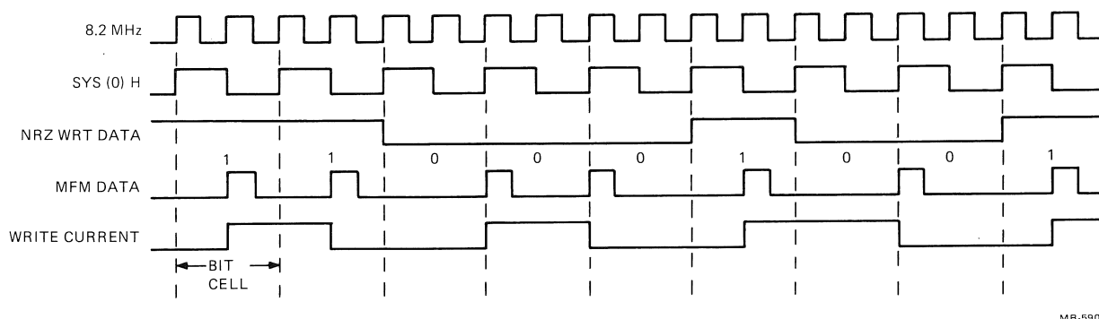
Figure 2-10 MFM Encoding
