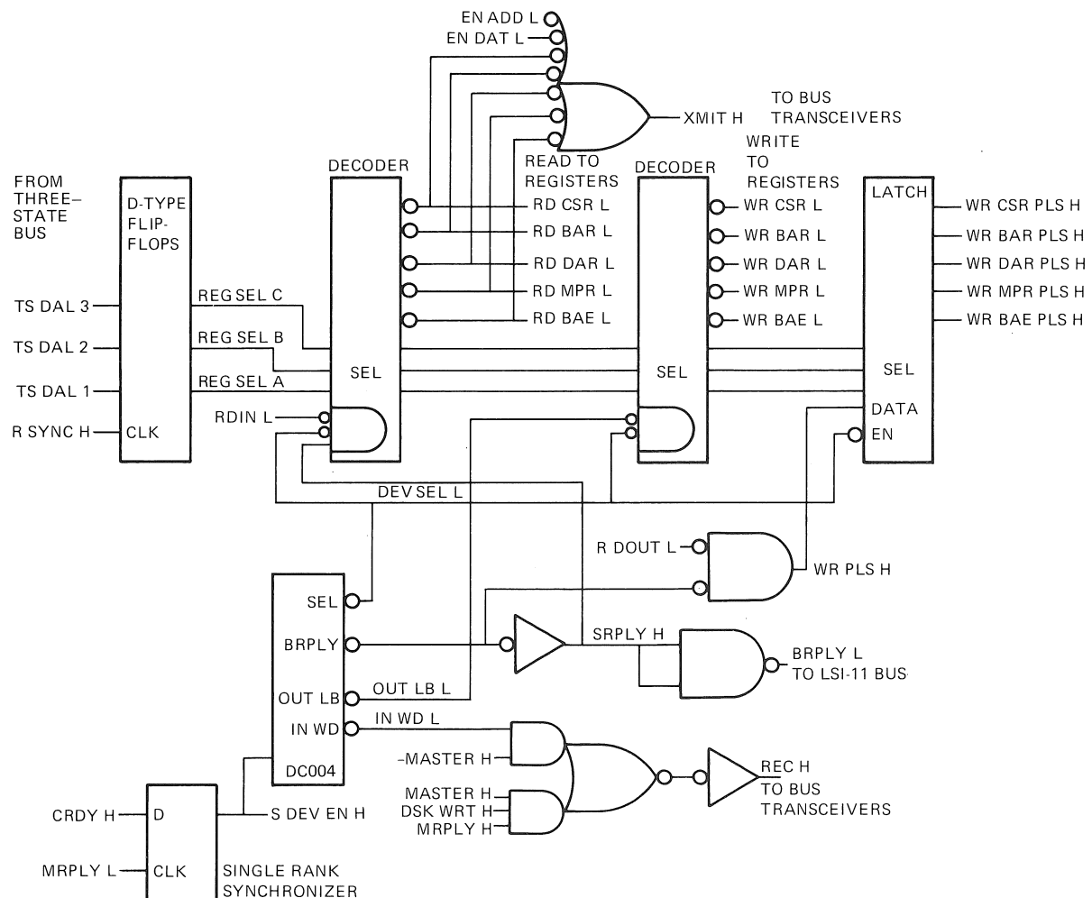
Figure 2-2 Bus Protocol Logic
