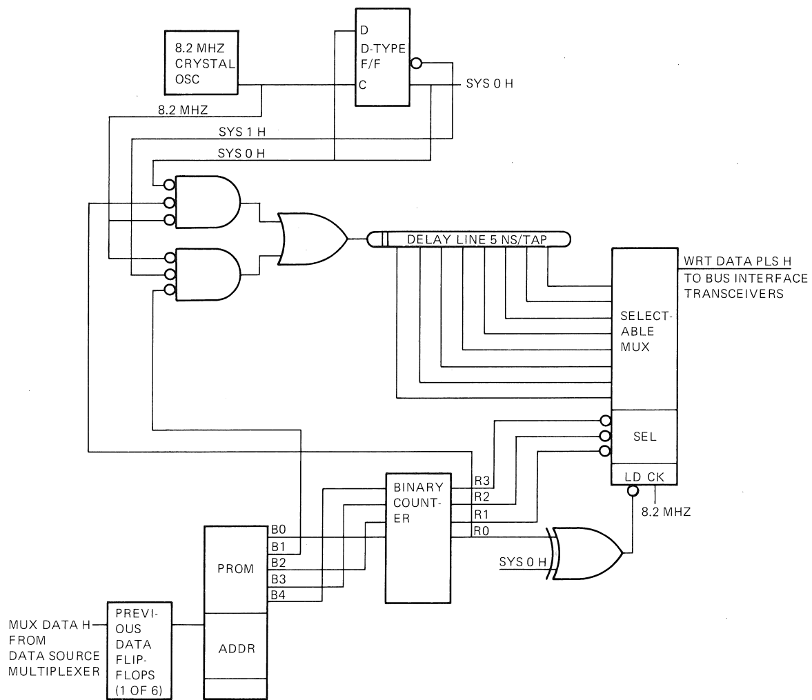
Figure 2-12 Write Encoder and Precompensation Circuit
