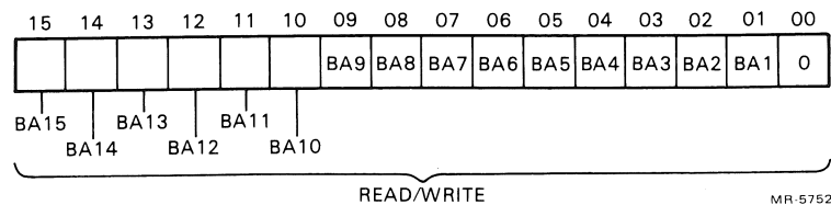
Figure 4-2 Bus Address Register (BAR)
