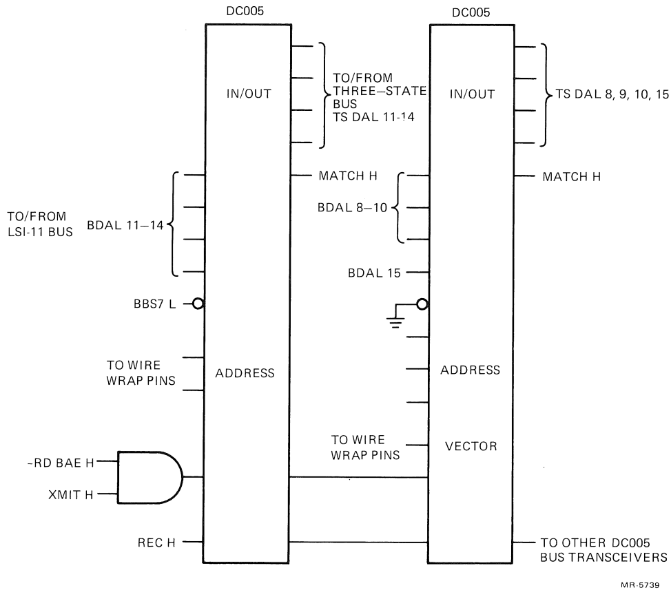
Figure 2-3 Bus Transceivers
