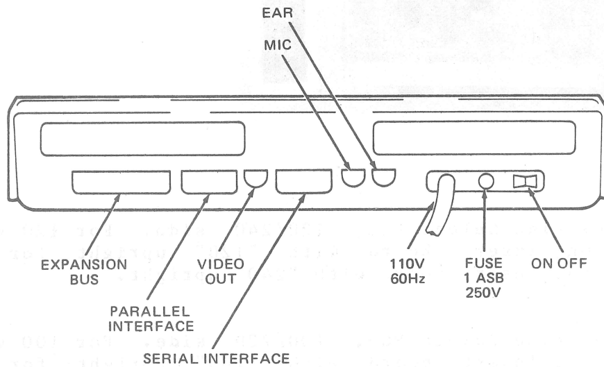
Rear of Sorcerer Computer
